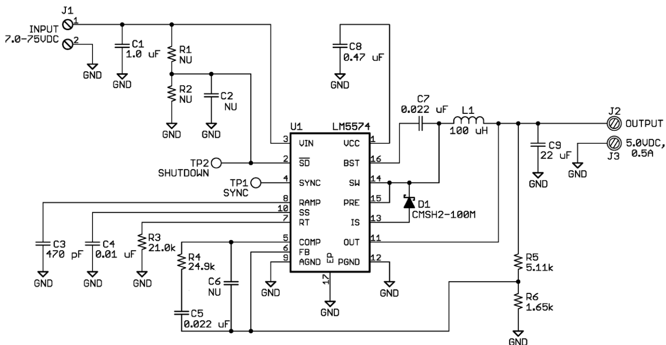
Figure 7-1. LM5574 Reference Schematic
