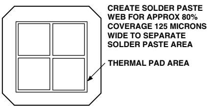
Figure 13. 5 mm × 5 mm LFSCP Solder Paste Mask Pattern
