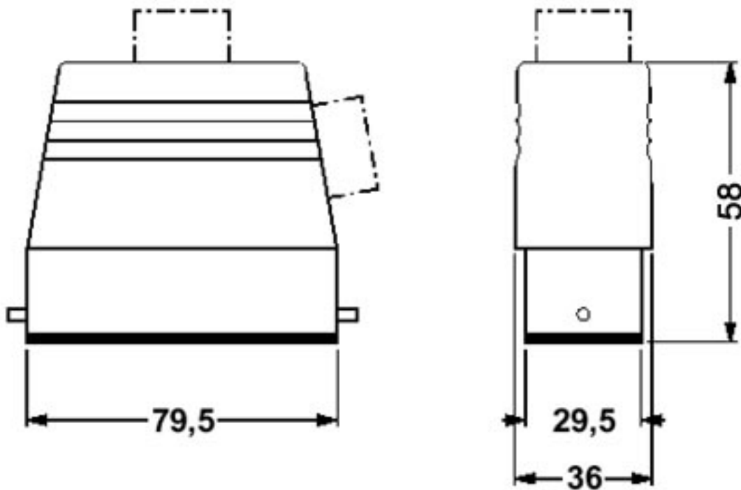
Dimensioned drawing
