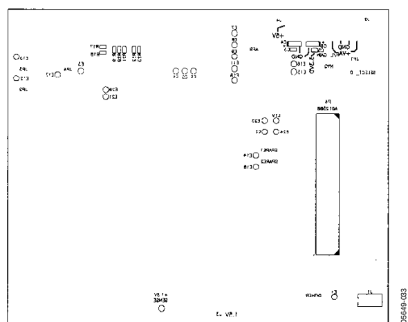
Figure 34. Bottom Silkscreen
