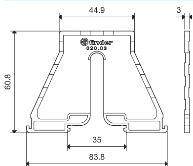
Separator for panel mounting, plastic, 3 mm wide
