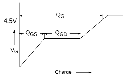
Fig 11b. Basic Gate Charge Waveform
