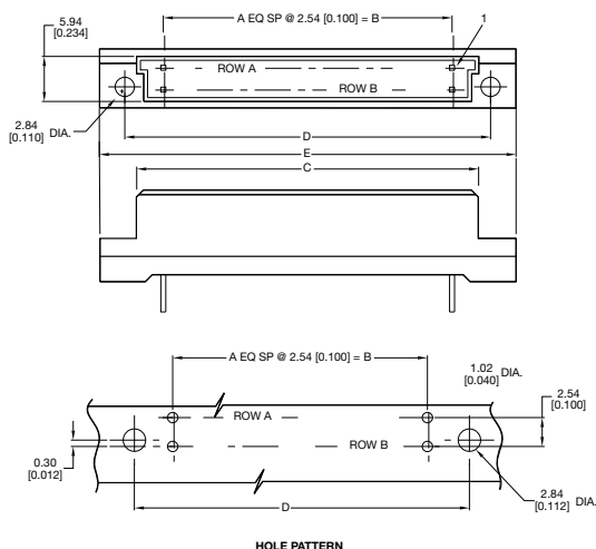
HOLE PATTERN
