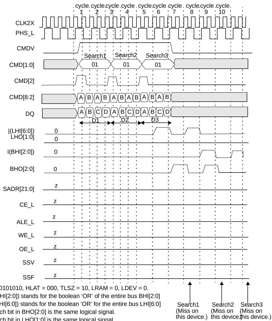
Figure 13-64. Timing Diagram for Devices Below the Winning Device in Block Number 3 Except Device Number 30 (the Last Device)
