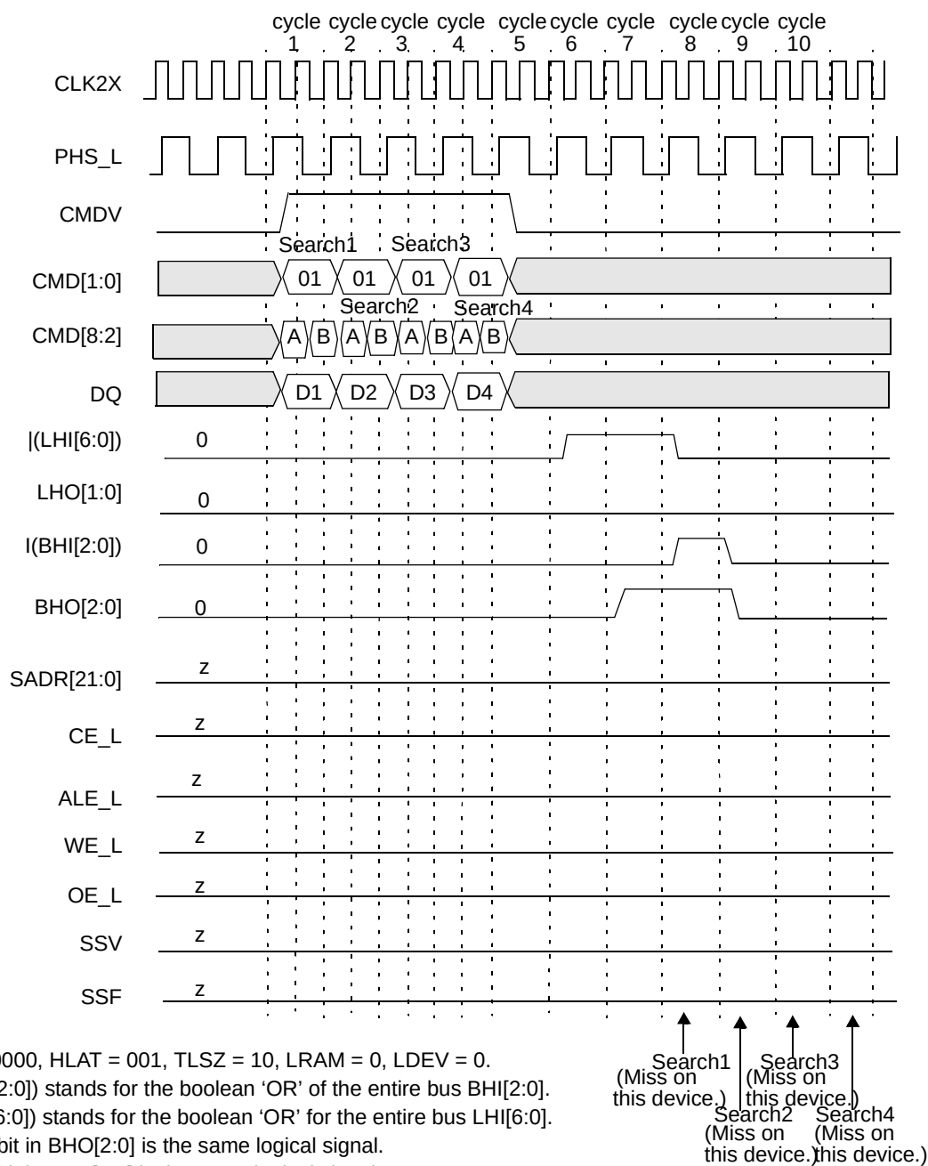
Figure 13-17. Timing Diagram for Devices Below the Winning Device in Block Number 2
