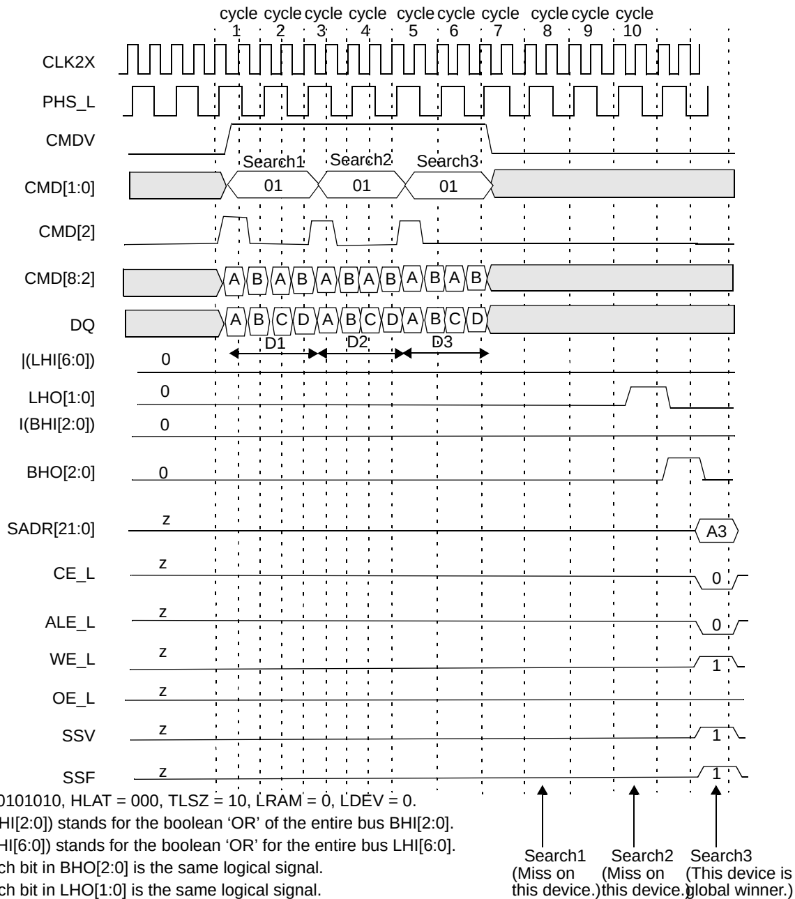
Figure 13-57. Timing Diagram for Globally Winning Device in Block Number 1
