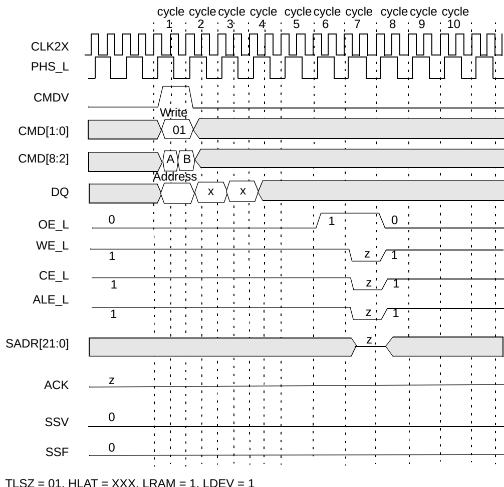
Figure 15-11. SRAM Write Timing for Device Number 7 in a Block of Eight Devices
