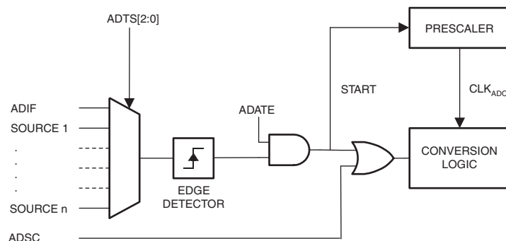
Figure 6-101. ADC Auto Trigger Logic
