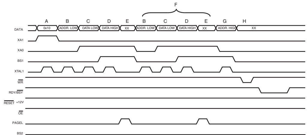
Figure 6-119. Programming the Flash Waveforms (1)
