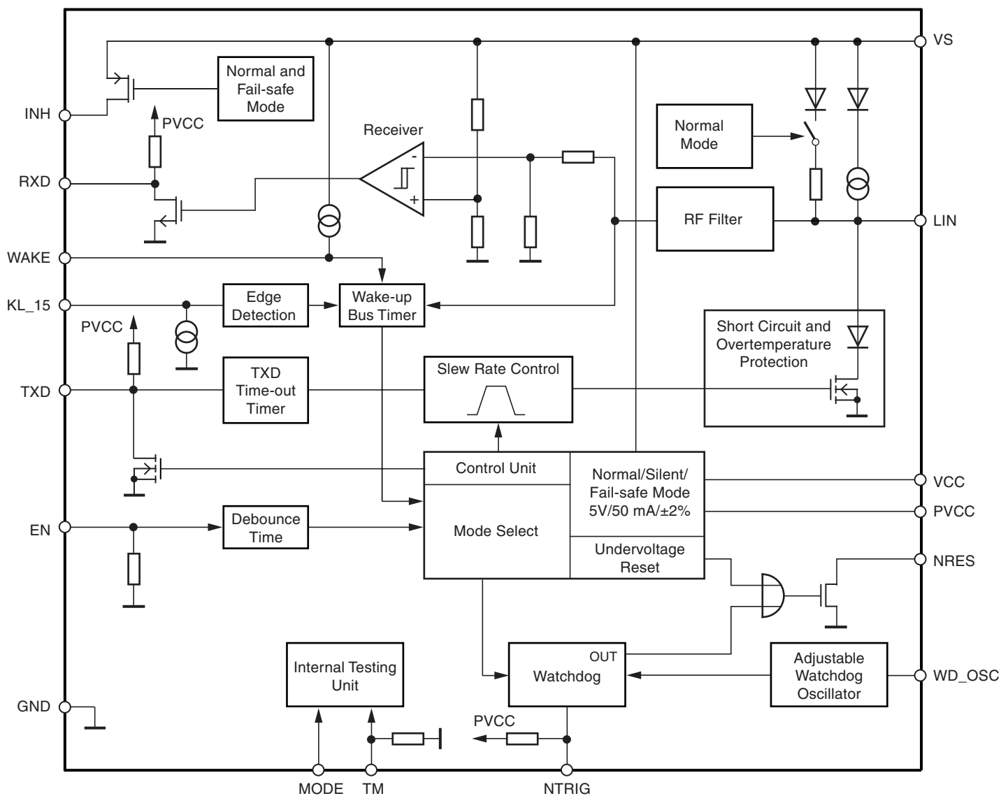
Figure 3-1. Block Diagram
