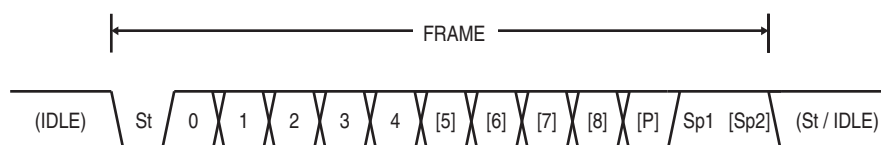
Figure 6-72. Frame Formats
