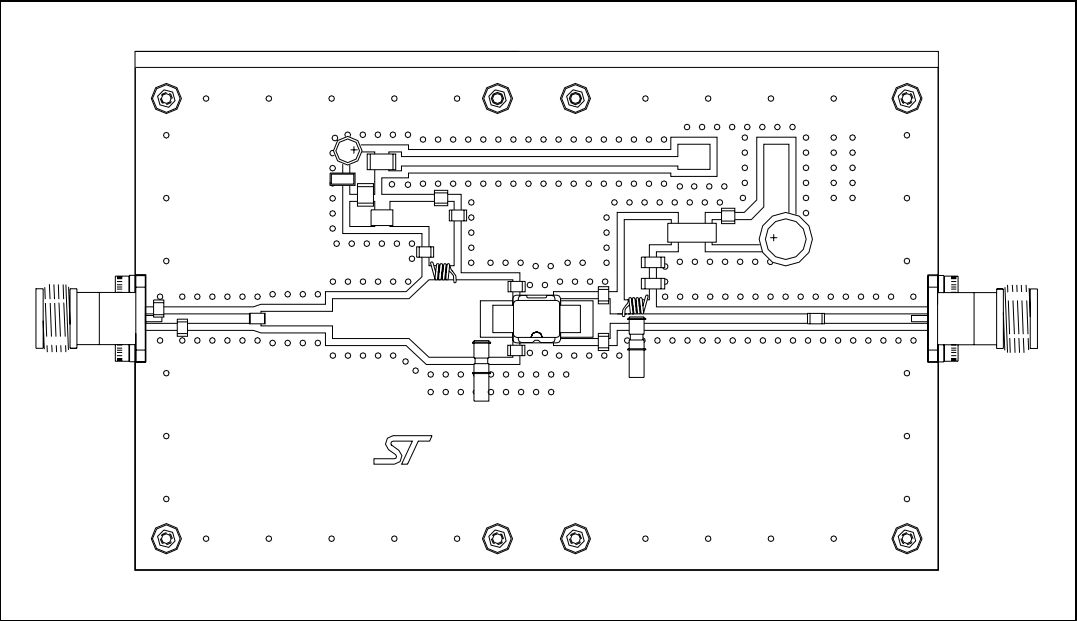
Figure 15. Test circuit
