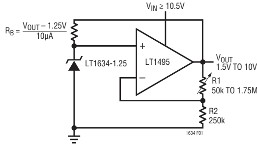
Figure 1. Adjustable Output Voltage Reference
