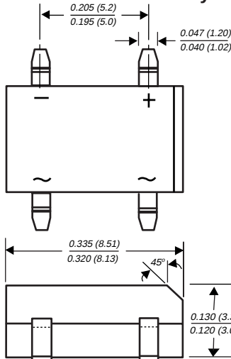
Case Style DFS
