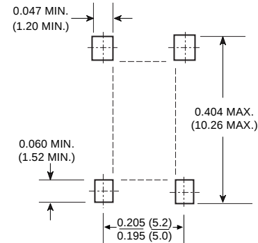
Mounting Pad Layout
