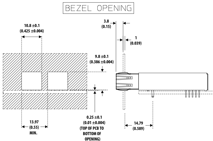
Figure 5. Recommended Board Layout Hole Pattern
