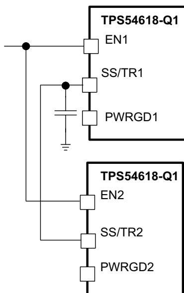
Figure 30. Schematic for Ratiometric Start-Up Sequence
