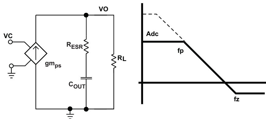
Figure 37. Simple Small-Signal Model and Frequency Response for Peak-Current-Mode Control
