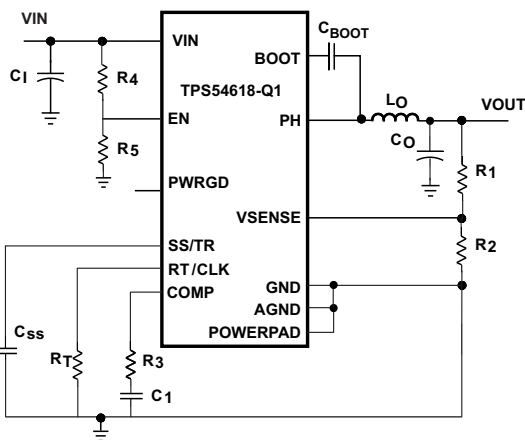
Figure 1. SIMPLIFIED SCHEMATIC
