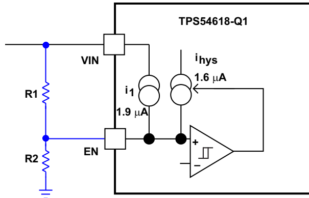
Figure 27. Adjustable Undervoltage Lockout
