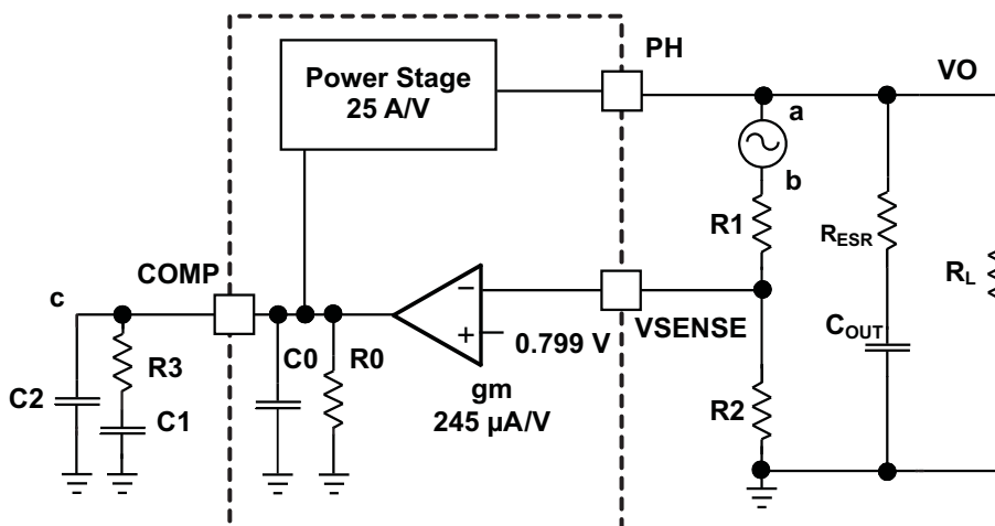
Figure 36. Small-Signal Model for Loop Response
