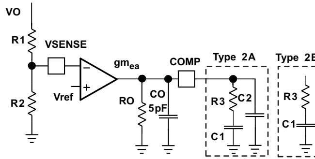
Figure 38. Types of Frequency Compensation
