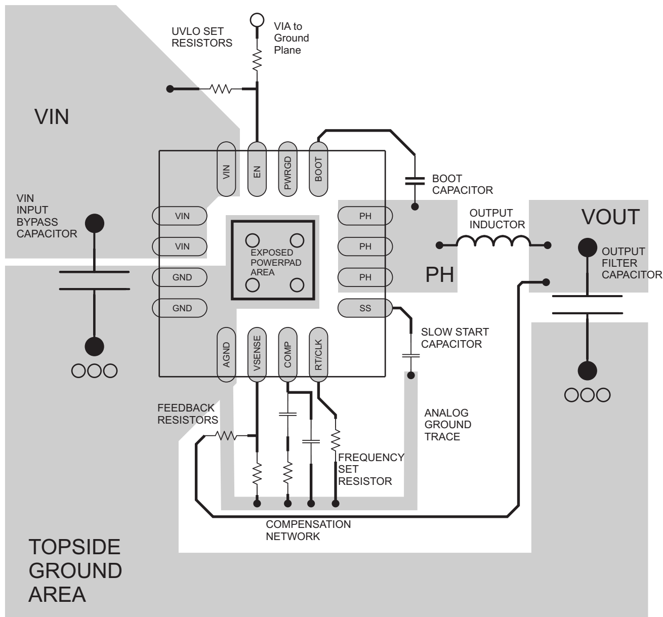
Figure 50. PCB Layout Example
