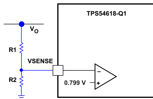
Figure 26. Voltage-Divider Circuit
