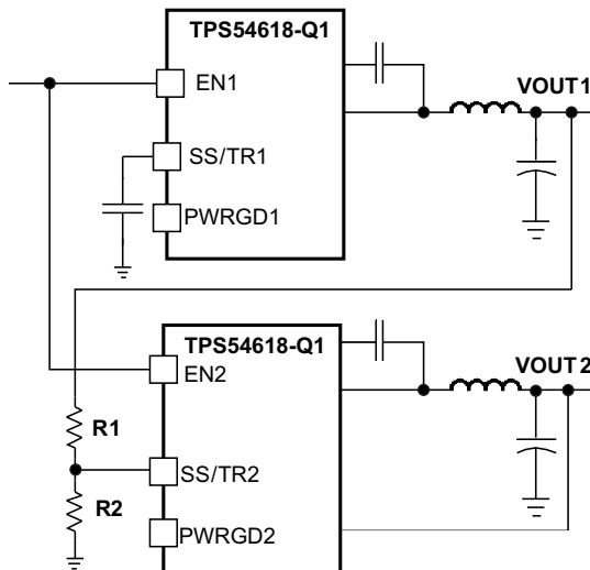
Figure 32. Ratiometric and Simultaneous Start-Up Sequence
