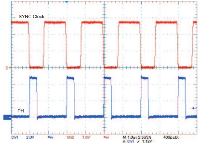
Figure 35. Plot of Synchronizing to System Clock
