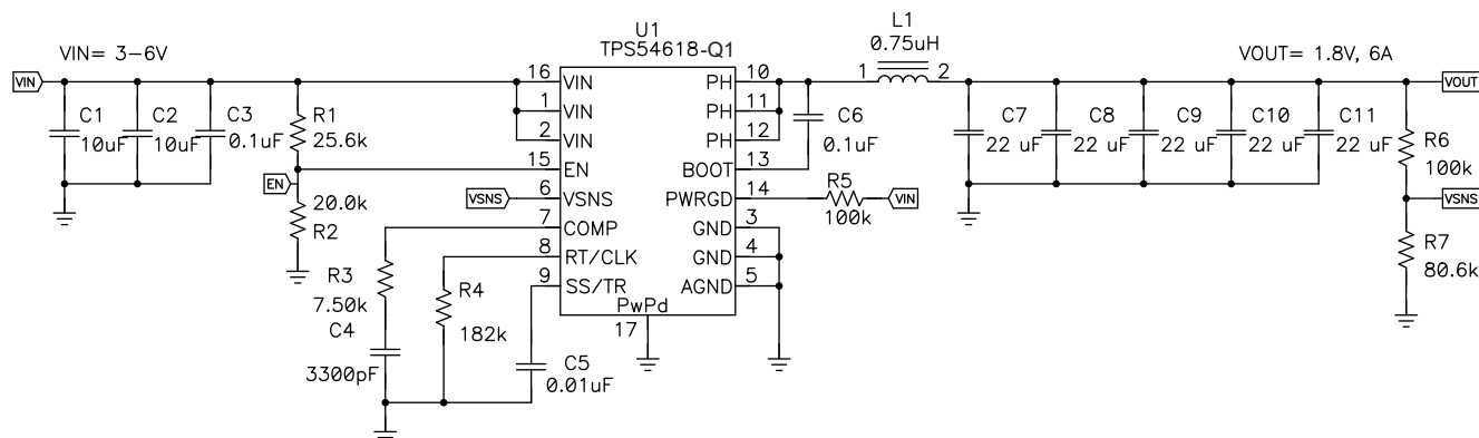
Figure 39. High Frequency, 1.8-V Output Power-Supply Design With Adjusted UVLO
