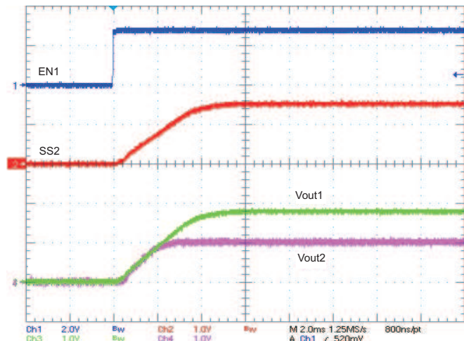
Figure 33. Ratiometric Start-Up Using Coupled SS/TR Pins
