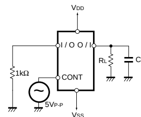
Fig. 8 Control IN→OUT crosstalk
