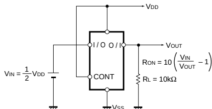
Fig. 2 ON resistance
