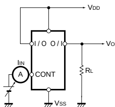
Fig. 1 Input voltage, current
