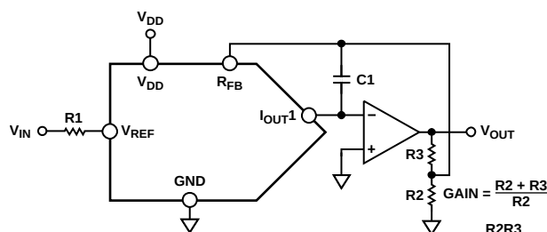
Figure 48. Increasing Gain of Current-Output DAC
