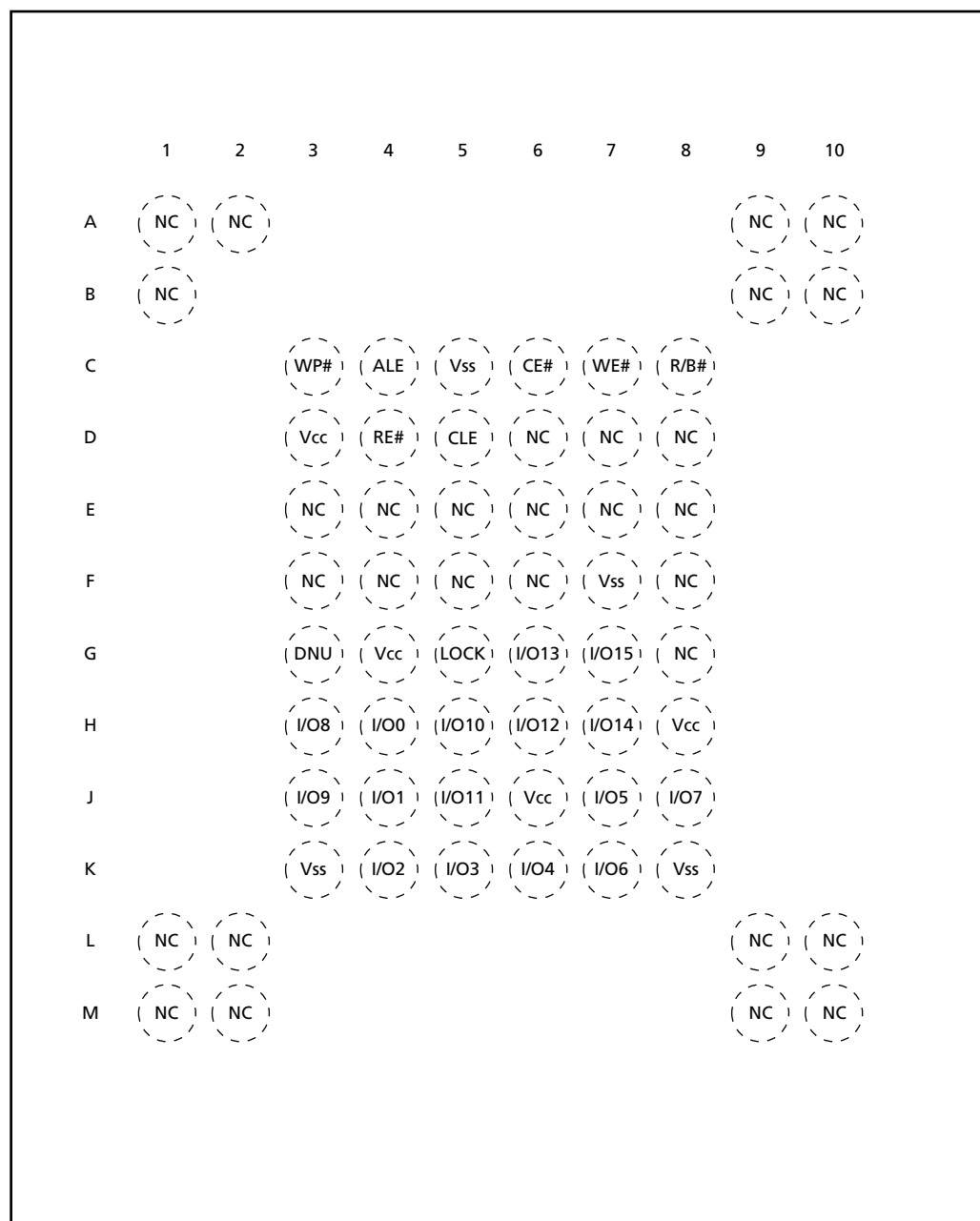
Figure 6: Ball Assignment: 63-Ball VFBGA (x16)
