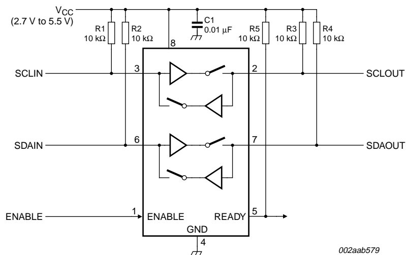
Fig 13. Typical application of PCA9514A
