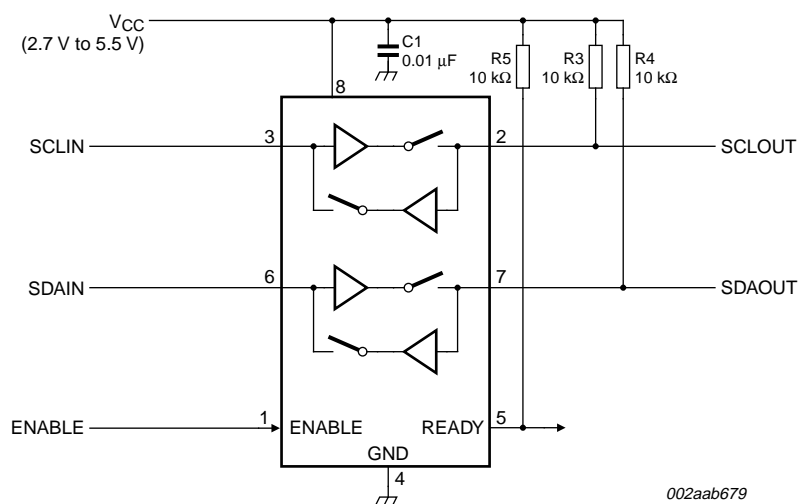
Fig 12. Typical application of PCA9513A
