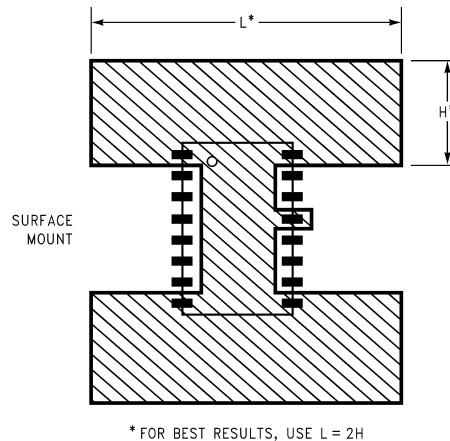
Figure 4. Heat Sink Foil Patterns
