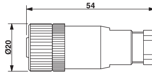
Dimensioned drawing
