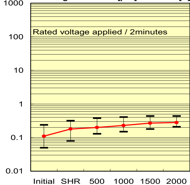
Leakage Current [μA] vs Time[h]
