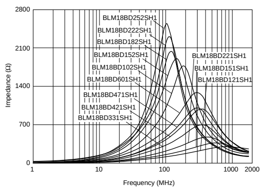
BLM18BD Series
