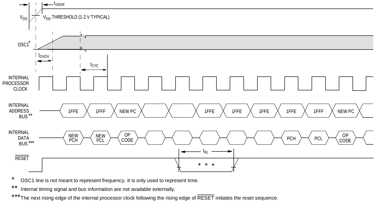
Figure 13-7. Power-On Reset and External Reset Timing Diagram
