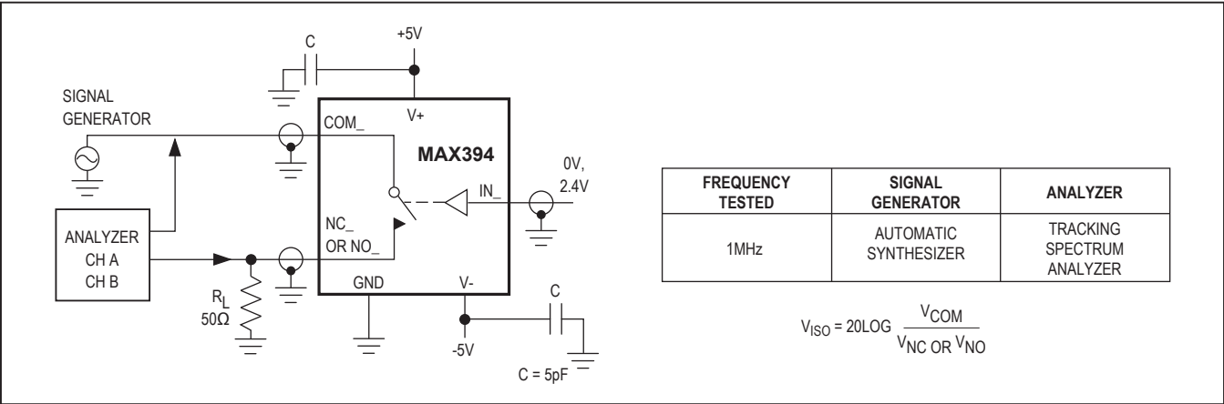
Figure 7. Off-Isolation
