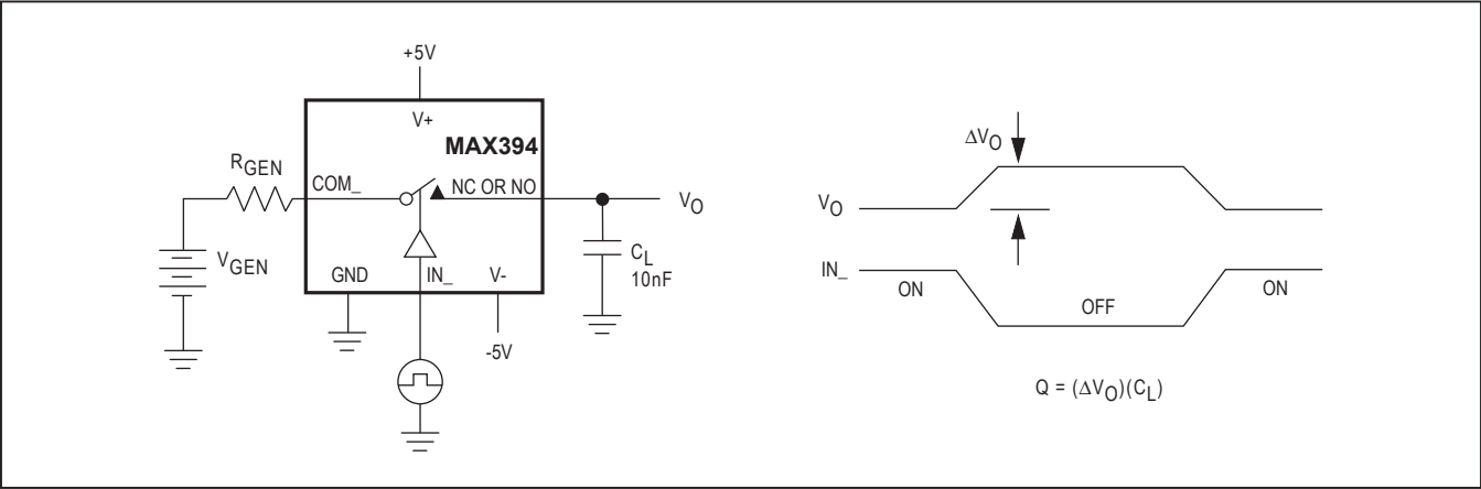
Figure 6. Charge Injection
