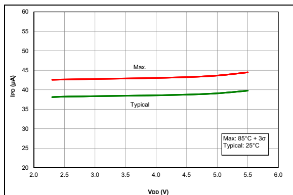
FIGURE 36-17: I PD , Fixed Voltage Reference (FVR), PIC16F18325/18345 Only
