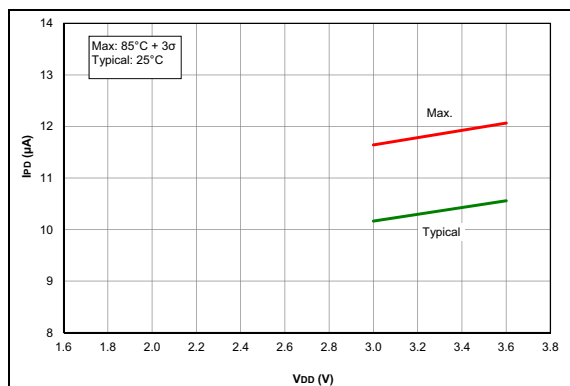
FIGURE 36-18: I PD , Brown-out Reset (BOR), BORV = 1, PIC16LF18325/18345 Only
