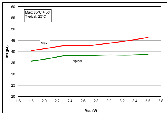
FIGURE 36-16: I PD , Fixed Voltage Reference (FVR), PIC16LF18325/18345 Only
