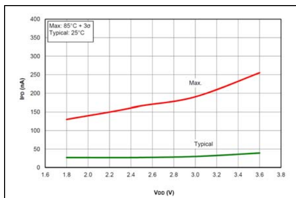
FIGURE 36-13: I PD BASE, Low-Power Sleep Mode, PIC16LF18325/18345 Only
