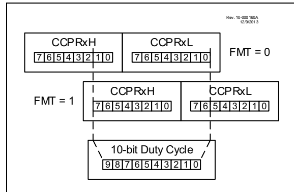
FIGURE 29-5: PWM 10-BIT ALIGNMENT BLOCK DIAGRAM
