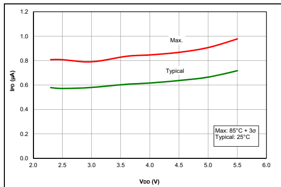
FIGURE 36-15: I PD , Watch Dog Timer (WDT), PIC16F18325/18345 Only
