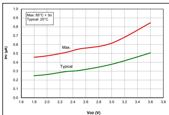
FIGURE 36-14: I PD , Watch Dog Timer (WDT), PIC16LF18325/18345 Only
