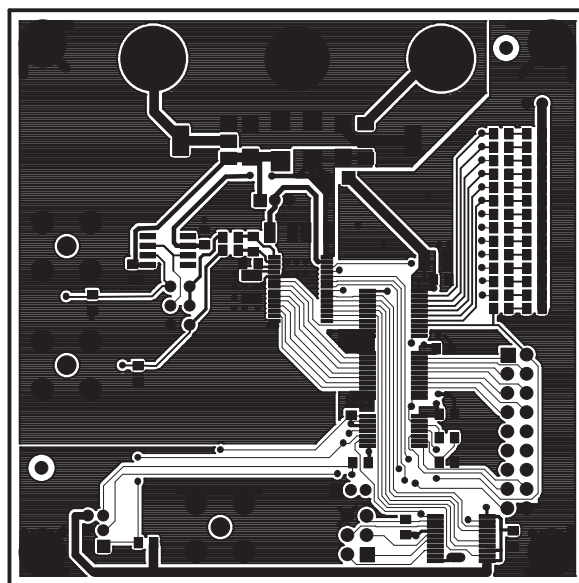
Figure 12c. Suggested Evaluation Circuit Board—Top Layer
