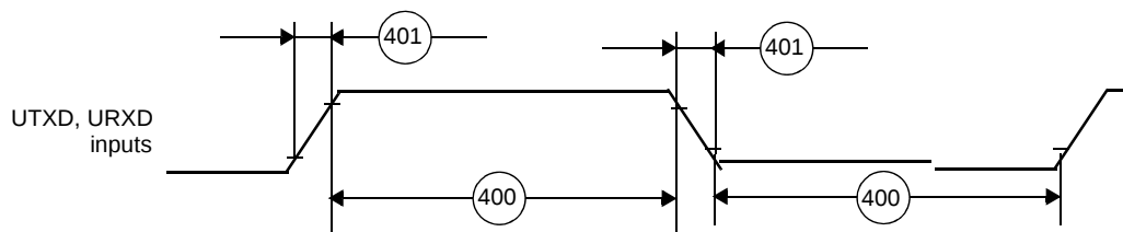
Figure 17. UART Input Timing
