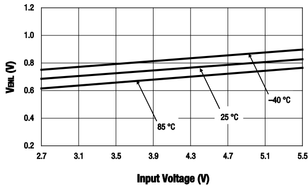
Figure 12. EN Input Low Threshold Voltage vs Input Voltage
