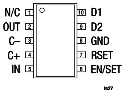
Figure 2. AAT3192 SC70JW-10 (Top View)
