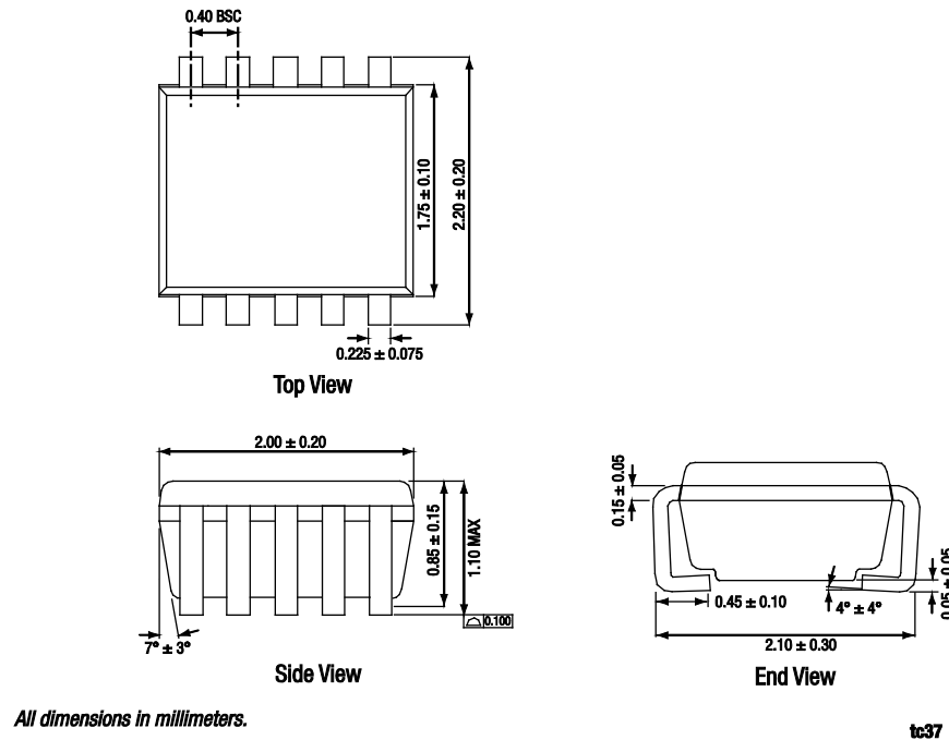
Figure 29. AAT3192 SC70JW-10 Package Dimensions
