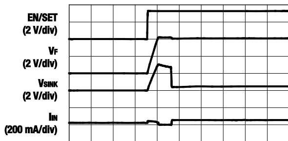
Figure 9. 1X Mode Turn On ( V_{IN} = 4.2 V, 19.6 mA/ch)
