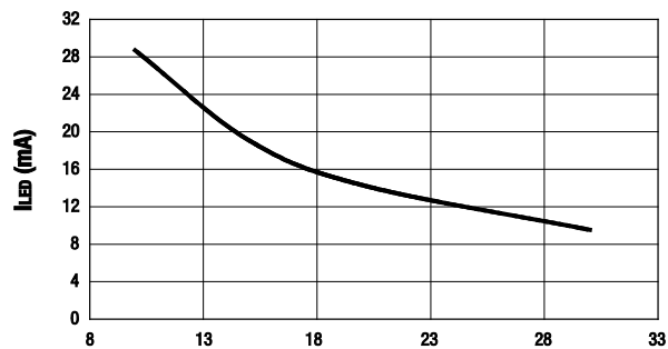
Figure 10. Maximum LED Current vs RSET
