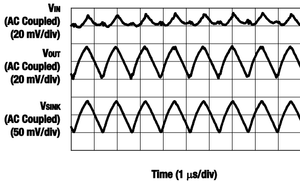
Figure 17. Output Ripple Waveform (2X Mode; 20 mA Load)
