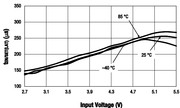
Figure 13. EN/SET Input Latch Timeout vs Input Voltage
