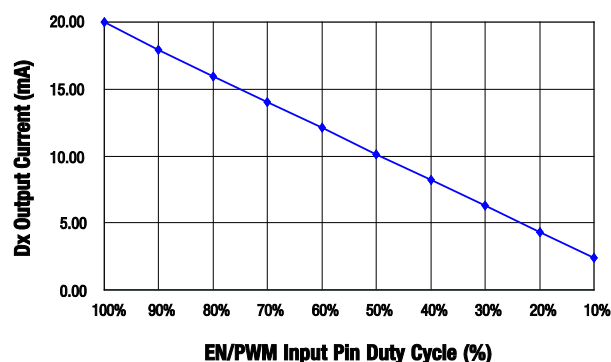
Figure 24. AAT3192-4 Current Control Profile (RSET = 14.3 kΩ, fPWM = 50 kHz)
