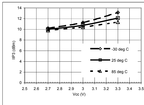
Figure 14. Cell CDMA LNA IIP3 (Mid Gain) at 881 MHz
