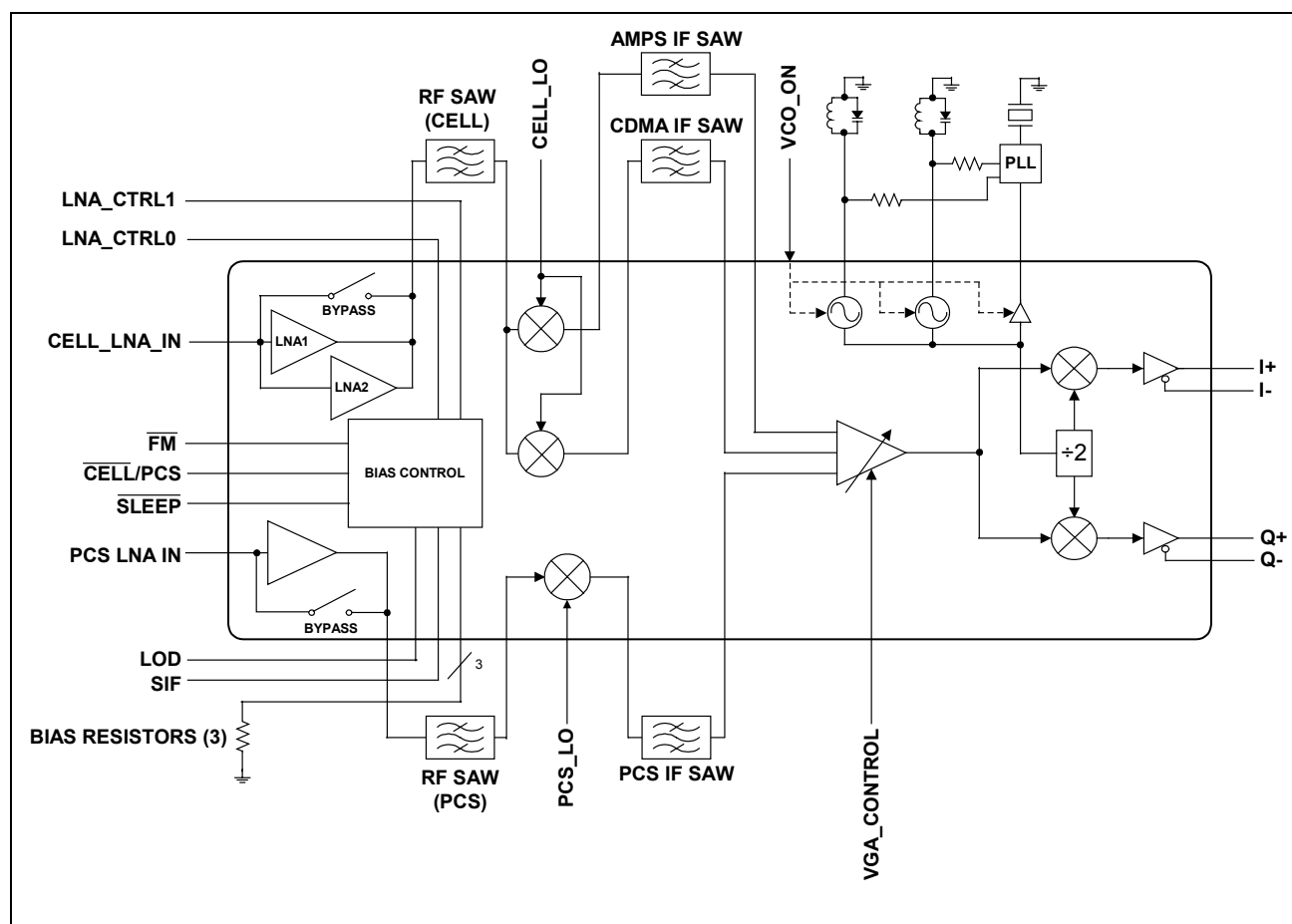
Figure 2. CX74001 Rx ASIC Block Diagram
