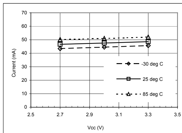
Figure 44. Supply Current in Cell CDMA Mode (LNA ON)
