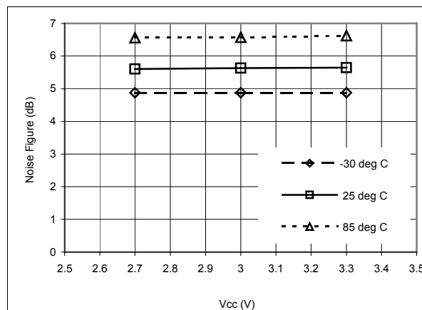
Figure 16. Cell CDMA LNA Noise Figure (Bypass Mode) at 881 MHz
