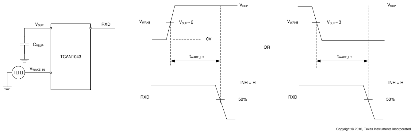
Figure 7-13. t_{Wake\_HT} While Monitoring RXD Output
