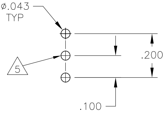
PCB HOLE LAYOUT
