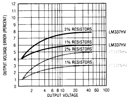
Worst Case Output Voltage Error @ T_J = 25^\circ\text{C}
