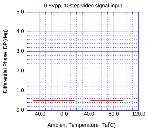
Differential Phase vs. Temperature
