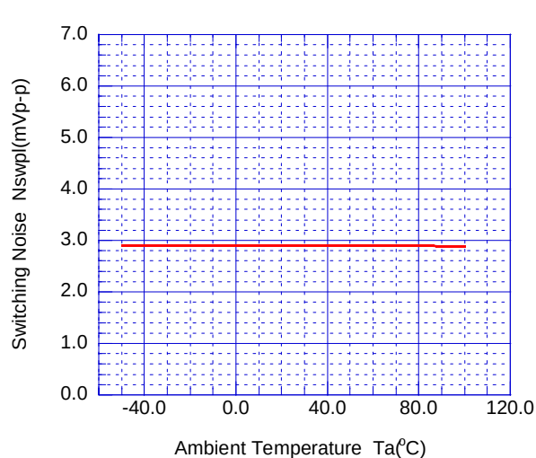
Switching Noise Level vs. Temperature
