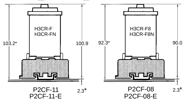
Dimensions with Front Connecting Socket P2CF-08-□/P2CF-11-□
