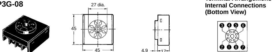
Terminal Arrangement/ Internal Connections (Bottom View)
