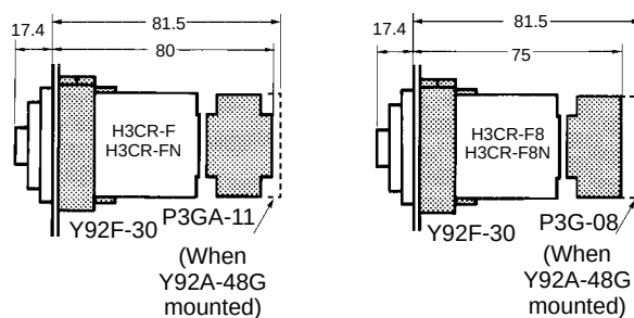
Dimensions with Back Connecting Socket P3G-08/P3GA-11
