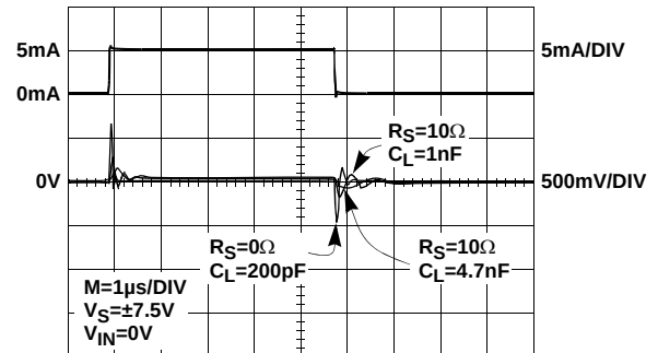
FIGURE 12. TRANSIENT LOAD REGULATION - SINKING (BUFFER)
