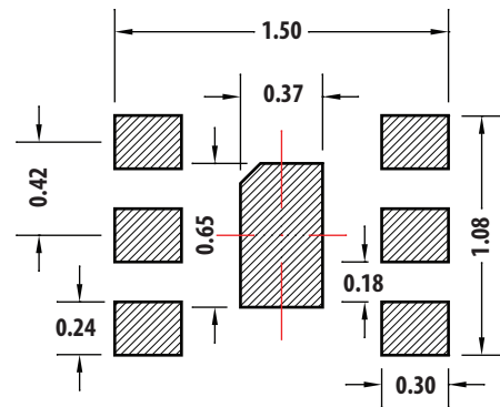
Stencil Opening
