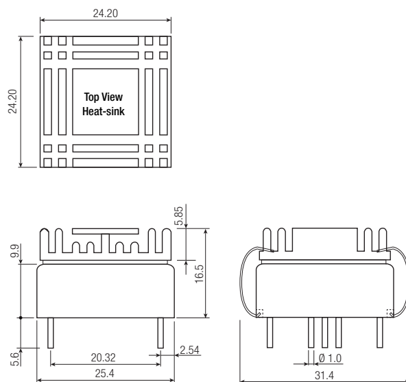
Dimension Drawing (mm) with Heat-sink
