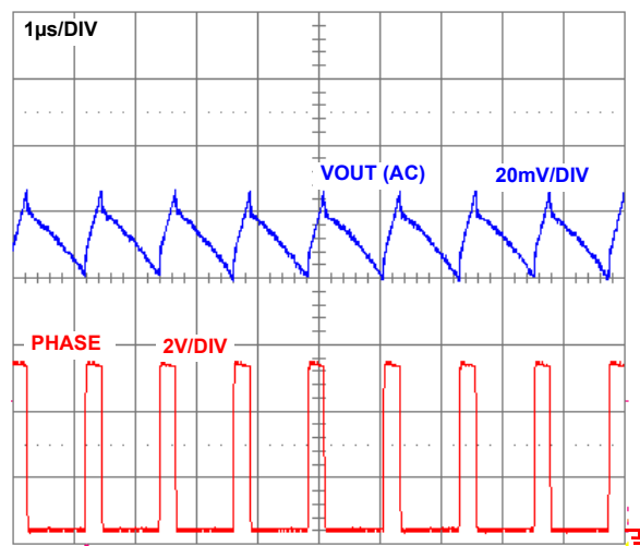
FIGURE 10. CCM STEADY-STATE
