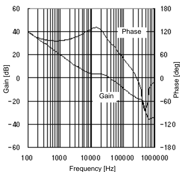
Figure 30. Gain vs Frequency 6 ( V_{CC}=6.0V , I_o=500mA )
