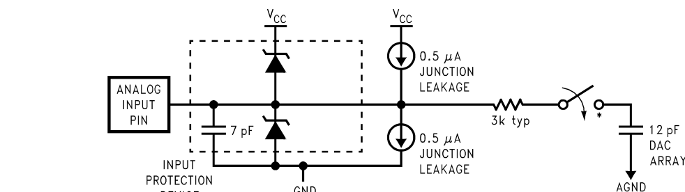
Figure 5-22. A/D Pin Model (Single Ended Mode)
