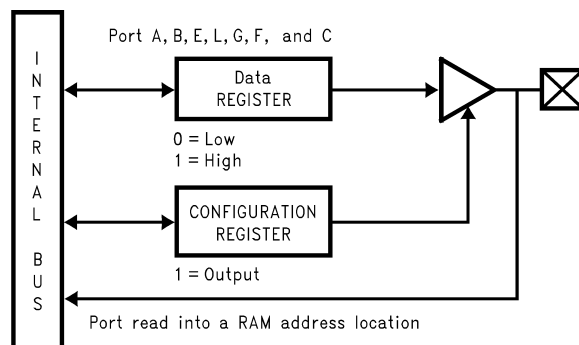
Figure 4-3. I/O Port Configurations—Output Mode
