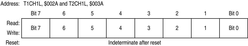
Figure 6-15. TIM Channel 1 Register Low (TCH1L)
