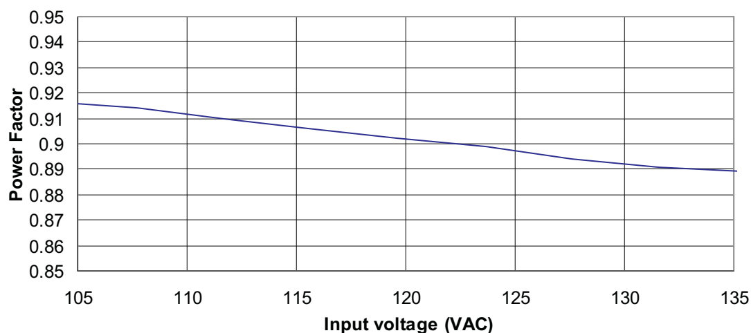
Figure 4. Input Voltage vs. Power Factor
