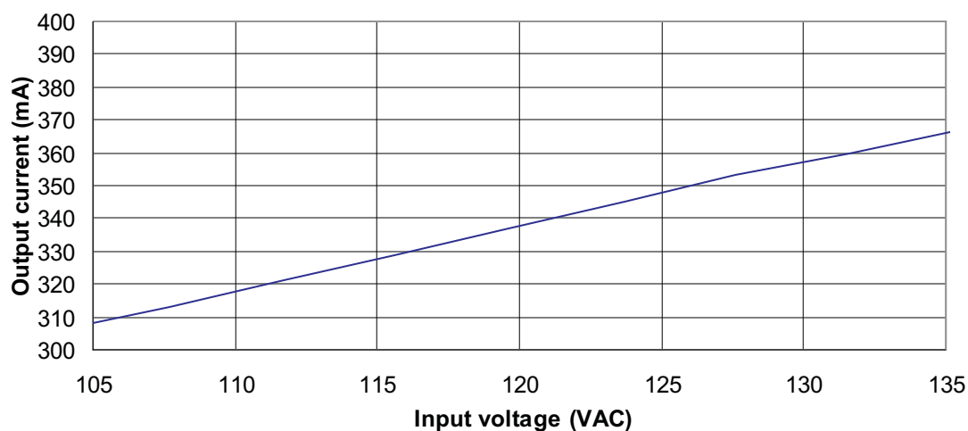
Figure 5. Output Current Variation (with respect to input voltage)
