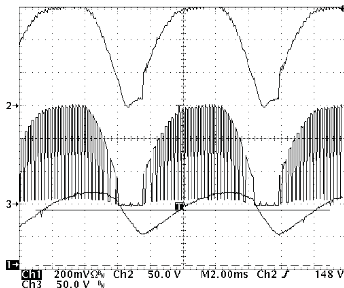
Figure 7. Output Ripple (Ch1-LED current Ch2- rectified line voltage Ch3- Q2 drain)
