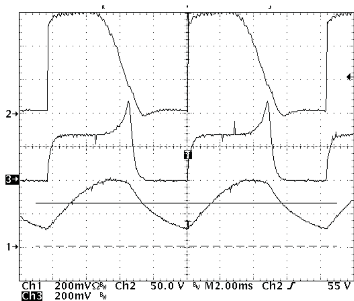
Figure 26. LED Current vs. Triac Conduction Time (Ch1- LED current Ch2- bulk voltage Ch3- U2-1 voltage waveform)
