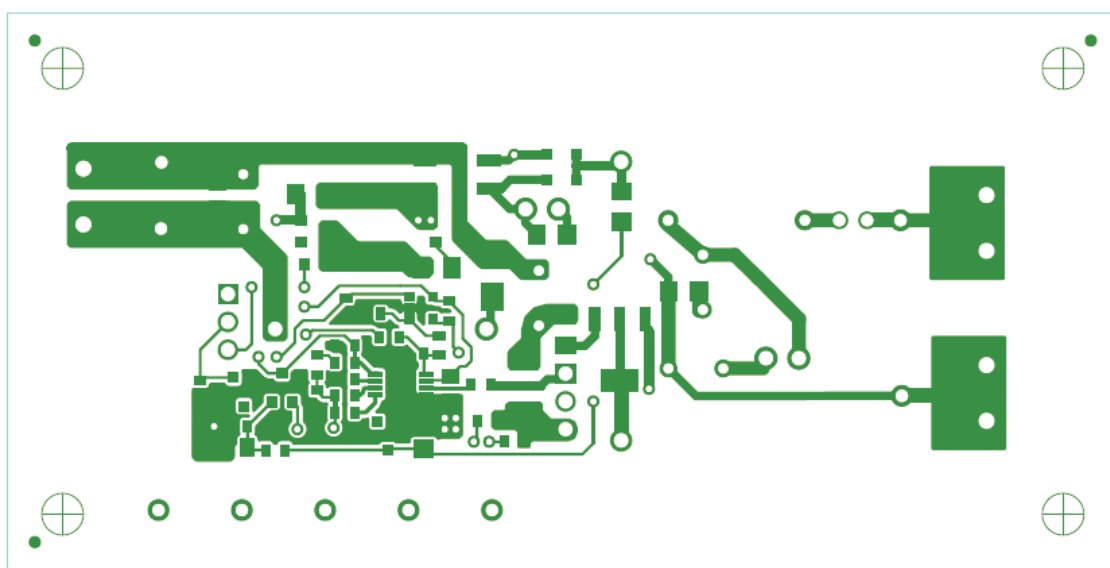
Figure 32. Bottom Copper (top view)
