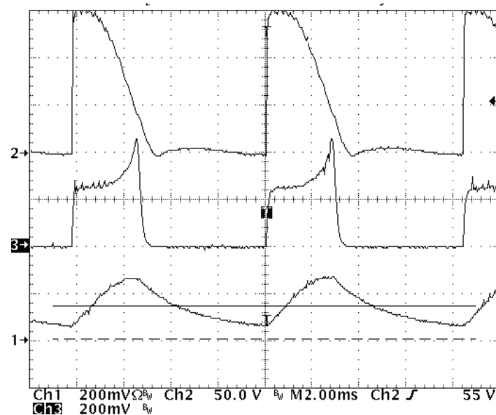
Figure 24. LED Current vs. Triac Conduction Time (Ch1- LED current Ch2- bulk voltage Ch3- U2-1 voltage waveform)
