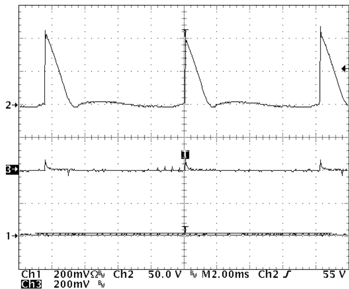
Figure 21. LED Current vs. Triac Conduction Time (Ch1- LED current Ch2- bulk voltage Ch3- U2-1 voltage waveform)
