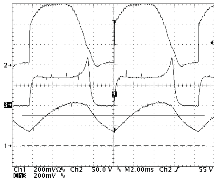
Figure 27. LED Current vs. Triac Conduction Time (Ch1- LED current Ch2- bulk voltage Ch3- U2-1 voltage waveform)
