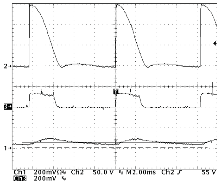
Figure 23. LED Current vs. Triac Conduction Time (Ch1- LED current Ch2- bulk voltage Ch3- U2-1 voltage waveform)
