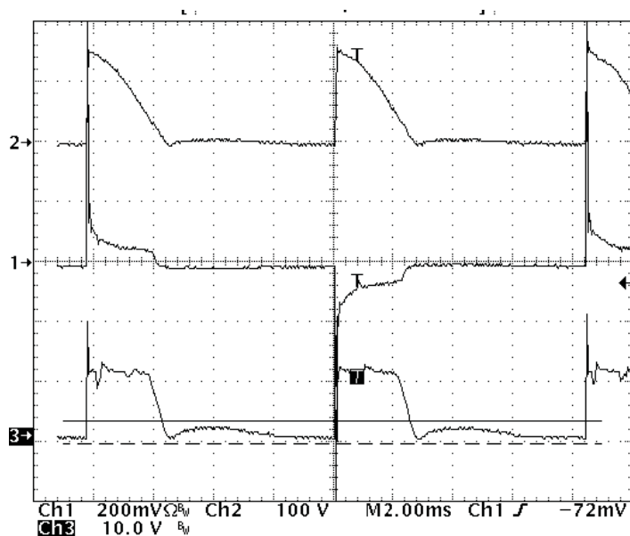
Figure 17. Dummy Load Conduction Time vs. Dimmer Setting (Ch1- line current Ch2- bulk voltage Ch3- Q4 source voltage )
