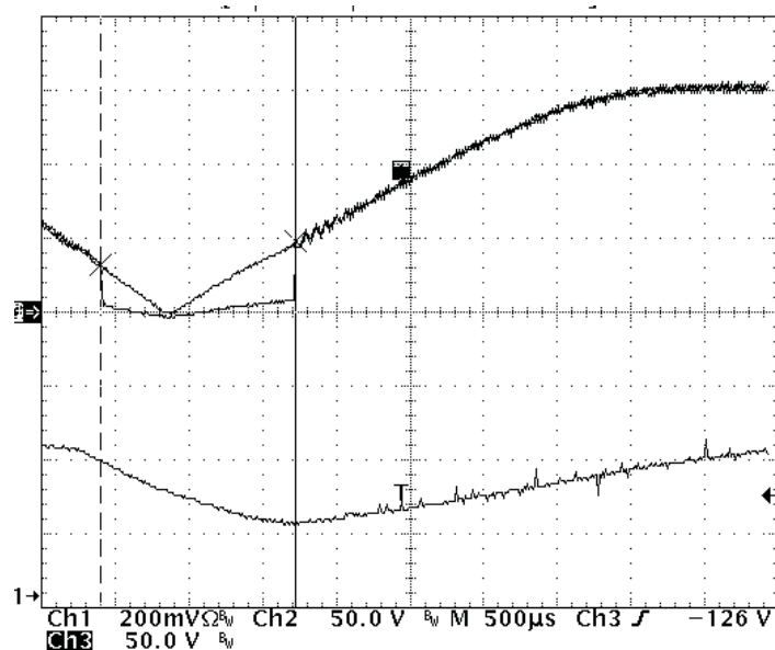
Figure 12. Dummy Load Conduction Time (Ch1- LED current Ch2- Q4 collector voltage Ch3- bulk voltage)
