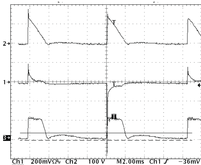
Figure 16. Dummy Load Conduction Time vs. Dimmer Setting (Ch1- line current Ch2- bulk voltage Ch3- Q4 source voltage)
