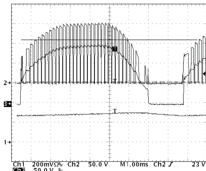
Figure 11. LED Current vs. Q2 Switch Node (Ch1- LED current Ch2- Q2 drain voltage Ch3- bulk voltage)
