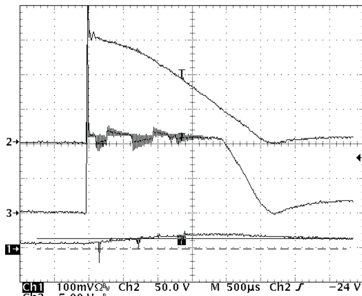
Figure 13. Triac Holding Current (2.5-ms Triac on time) (Ch1- LED current Ch2- bulk voltage Ch3- Q4 source voltage)
