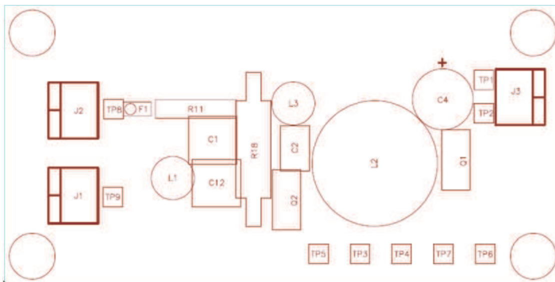
Figure 29. Assembly Drawing (top view)
