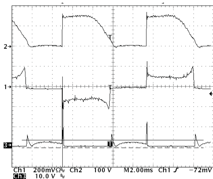
Figure 19. Dummy Load Conduction Time vs. Dimmer Setting (Ch1- line current Ch2- bulk voltage Ch3- Q4 source voltage )
