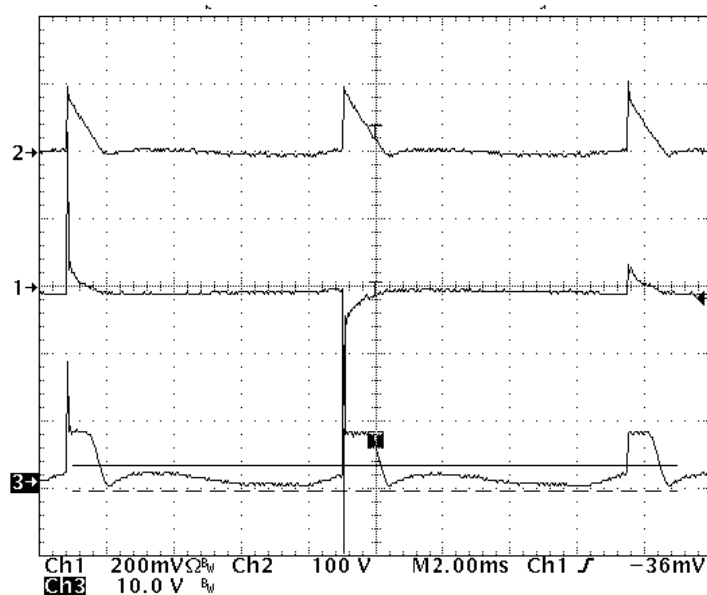
Figure 15. Dummy Load Conduction Time vs. Dimmer Setting (Ch1- Line current Ch2- bulk voltage Ch3- Q4 source voltage)
