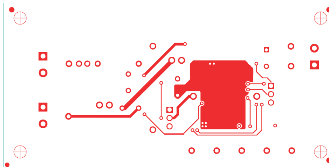
Figure 31. Top Copper (top view)
