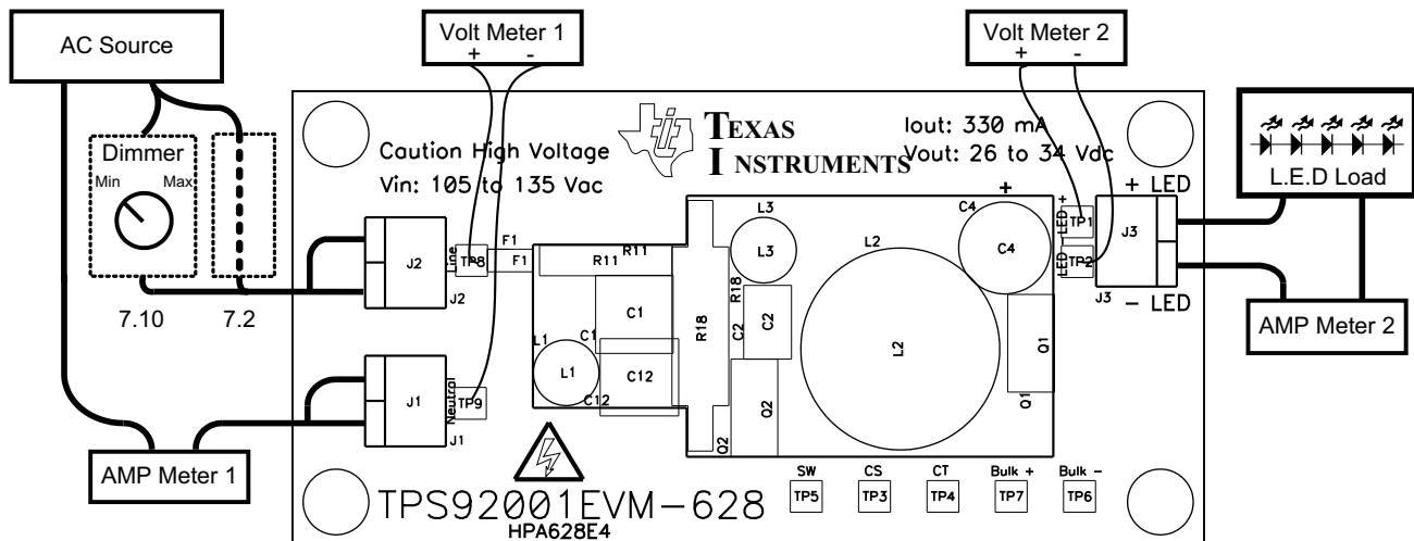
Figure 2. Recommended Test Set Up
