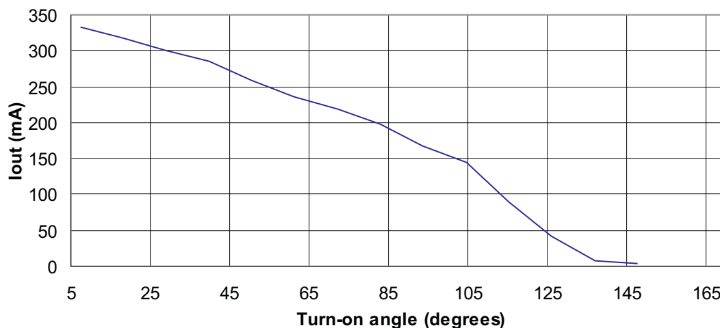
Figure 6. Output Current variation (with respect to input voltage phase)
