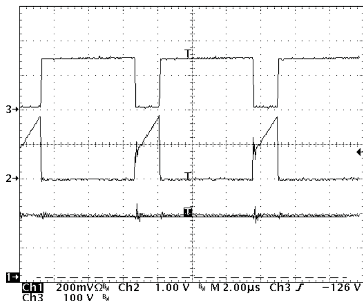
Figure 9. Current Sense and Switching Node Waveform (peak line) (Ch1- LED current Ch2- Q2 current sense Ch3- Q2 drain voltage)
