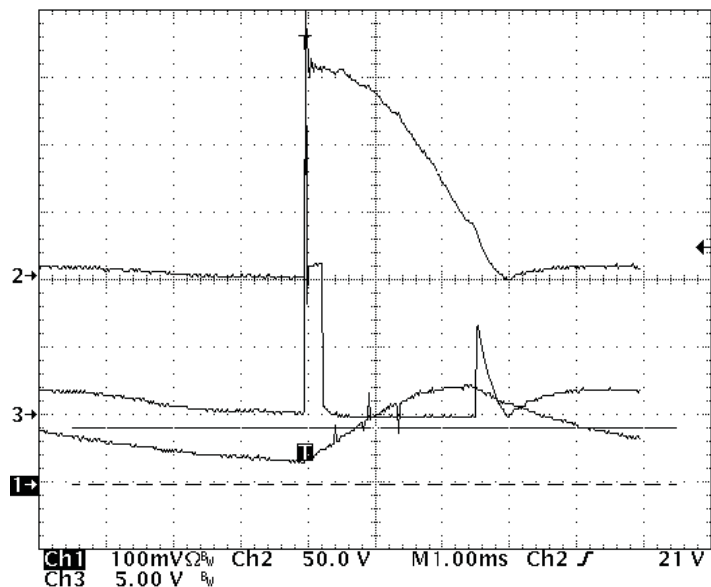
Figure 14. Triac Holding Current (3-ms Triac on time) (Ch1- LED current Ch2- bulk voltage Ch3- Q4 source voltage)
