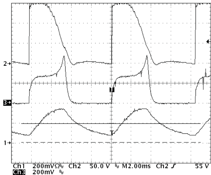
Figure 25. LED Current vs. Triac Conduction Time (Ch1- LED current Ch2- bulk voltage Ch3- U2-1 voltage waveform)
