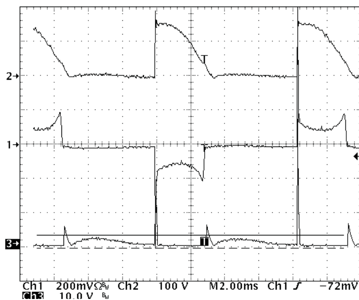
Figure 18. Dummy Load Conduction Time vs. Dimmer Setting (Ch1- line current Ch2- bulk voltage Ch3- Q4 source voltage )
