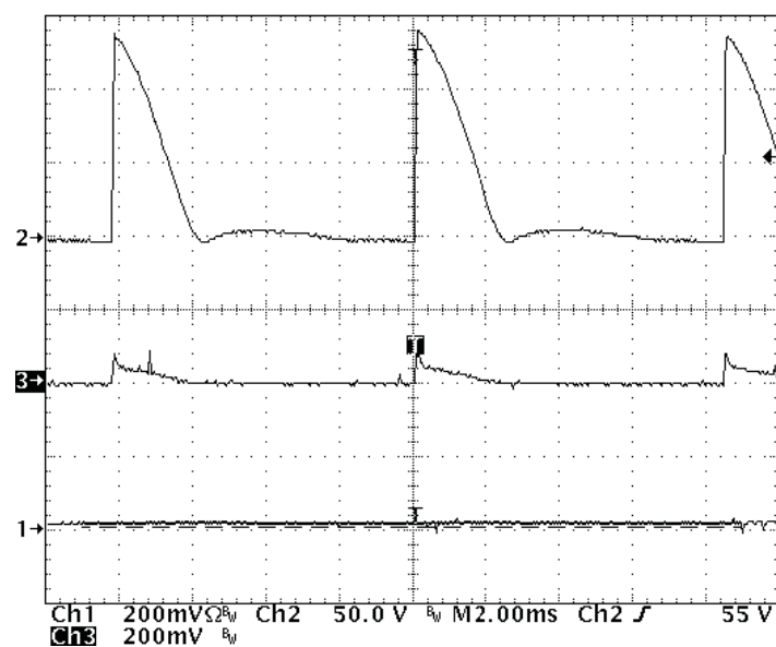
Figure 22. LED Current vs. Triac Conduction Time (Ch1- LED current Ch2- bulk line voltage Ch3- U2-1 voltage waveform)
