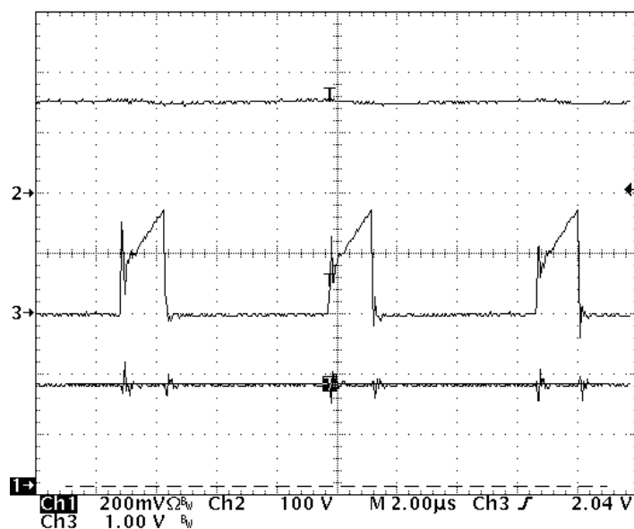
Figure 10. Line Voltage and Current Sense Waveform (peak line) (Ch1- LED current Ch2- AC line voltage Ch3- Q2 current sense)
