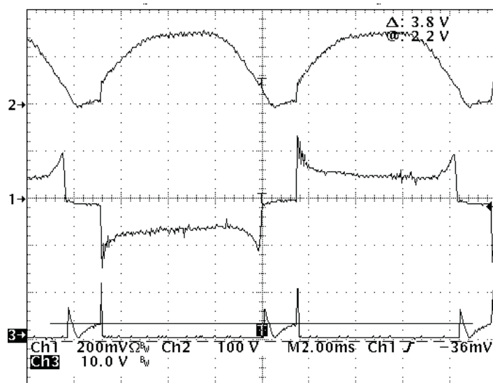
Figure 8. Input Waveform (Ch1- line current Ch2-rectified line voltage Ch3-Q4 source voltage)
