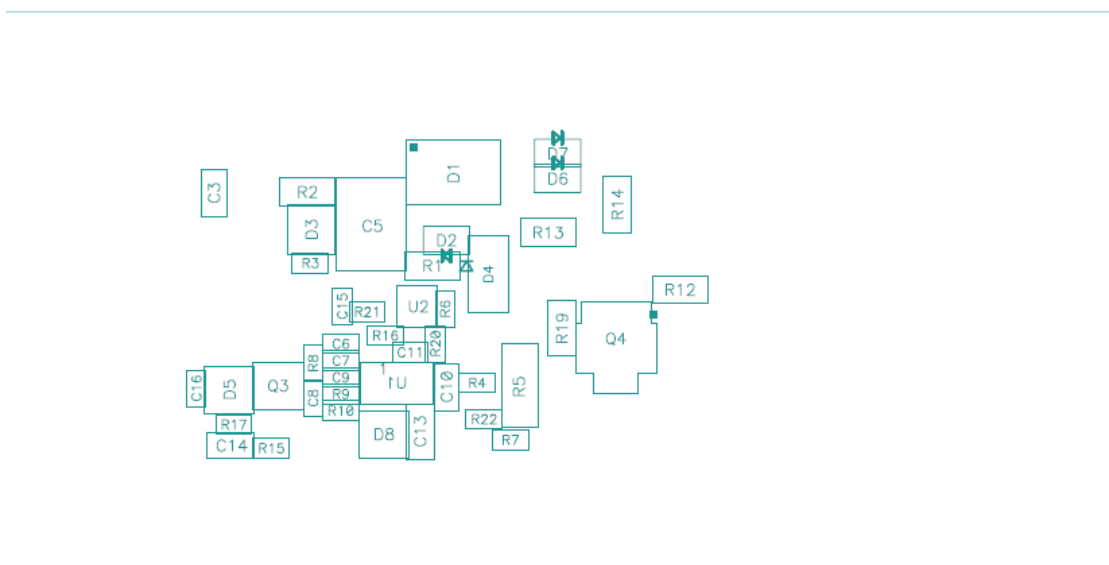
Figure 30. Assembly Drawing (bottom view)
