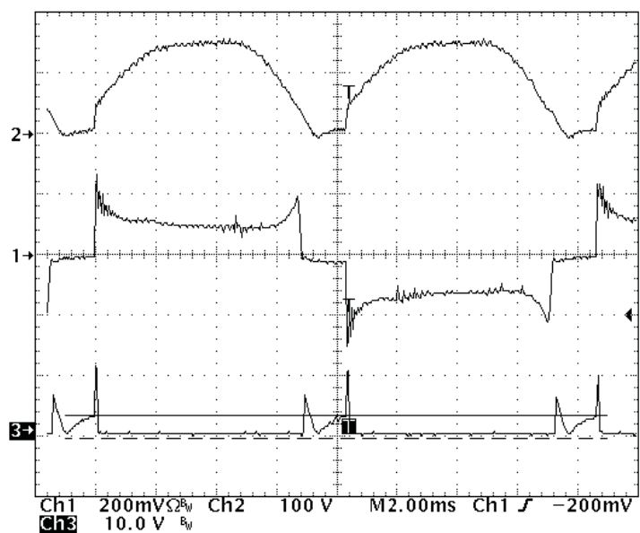
Figure 20. Dummy Load Conduction Time vs. Dimmer Setting (Ch1- line current Ch2- bulk voltage Ch3- Q4 source voltage)
