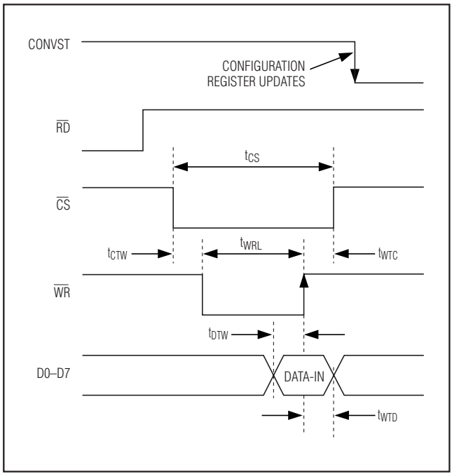
Figure 6. Write Timing
