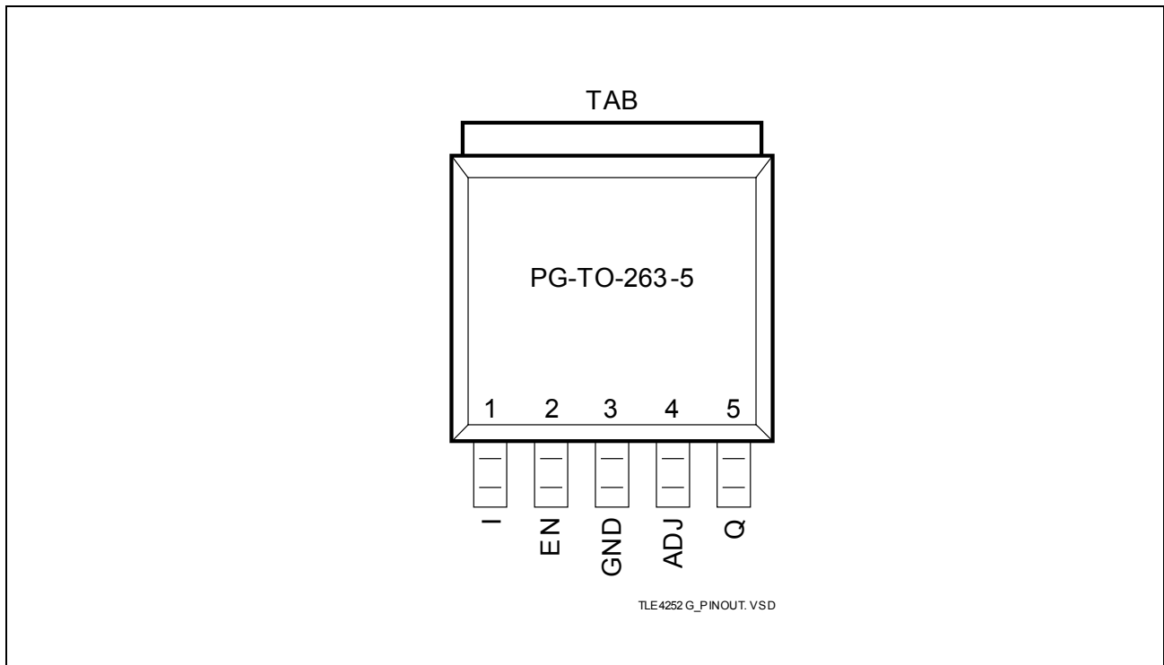
Figure 2 Pin Configuration
