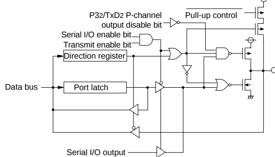
(5) Port P32
