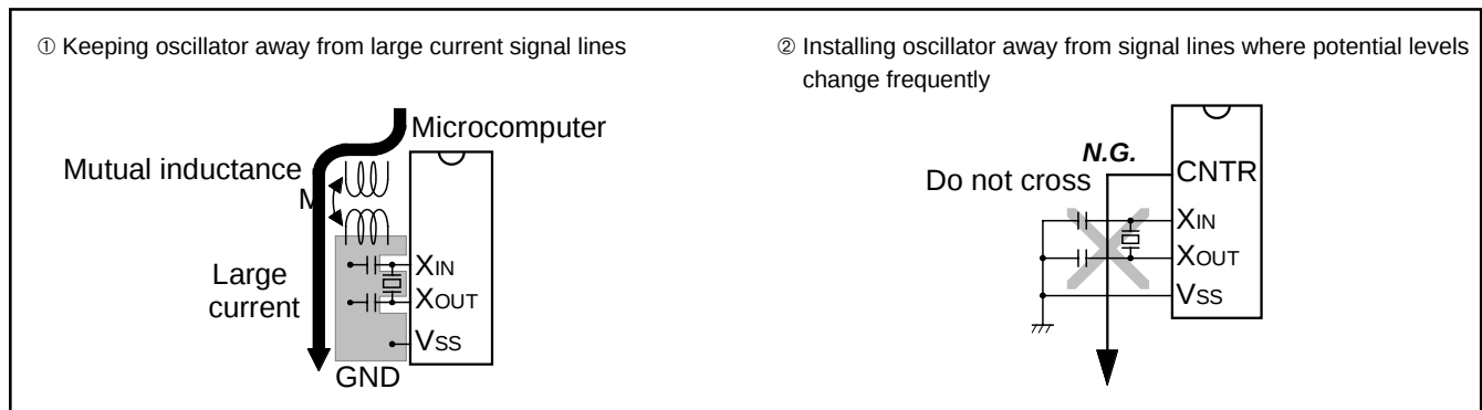
Fig. 59 Wiring for a large current signal line/Wiring of signal lines where potential levels change frequently
