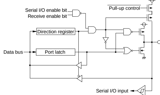
(6) Port P33
