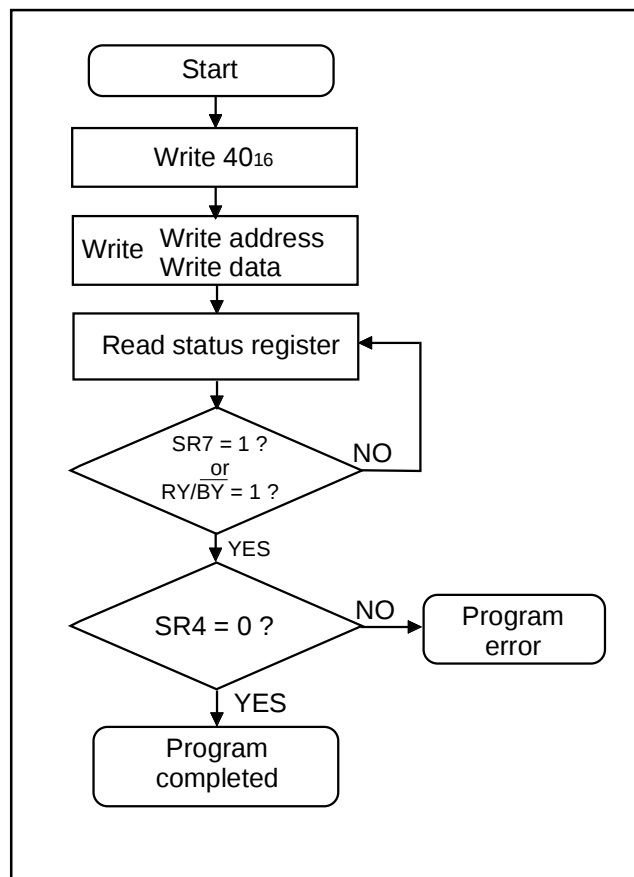
Fig. 64 Program flowchart
