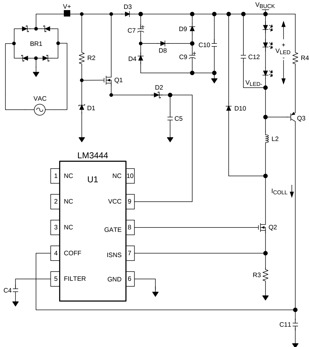
Figure 8. LM3444 Schematic
