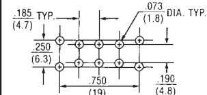
2 Pole P.C. Mounting
