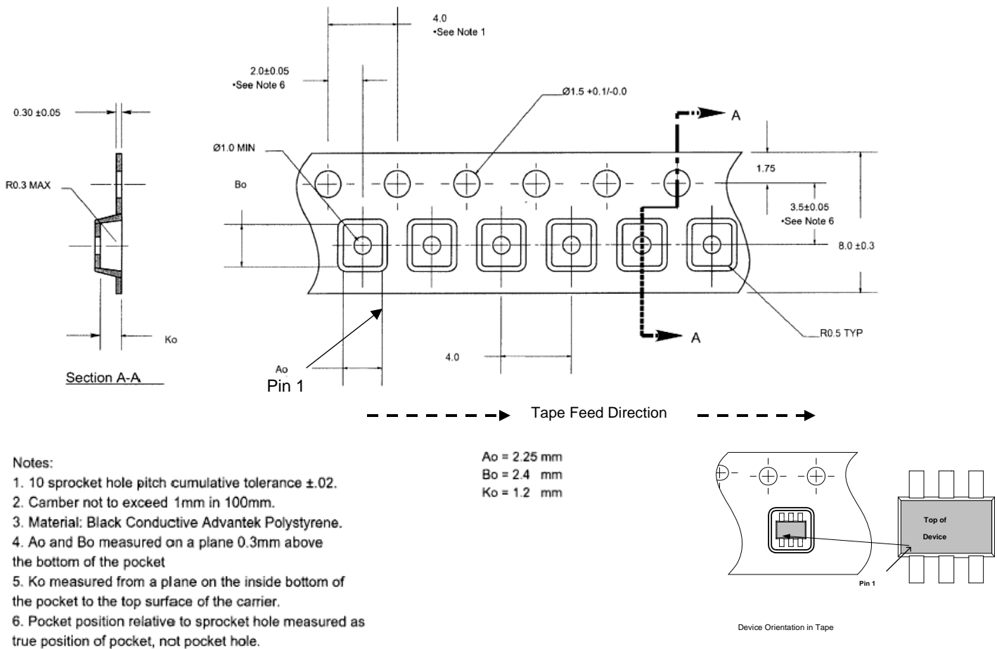
Figure 17. Tape and Reel Specifications
