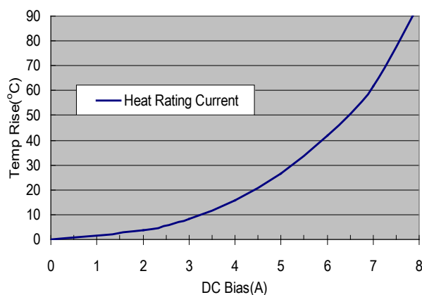
ASPI-0520LR-3R3
