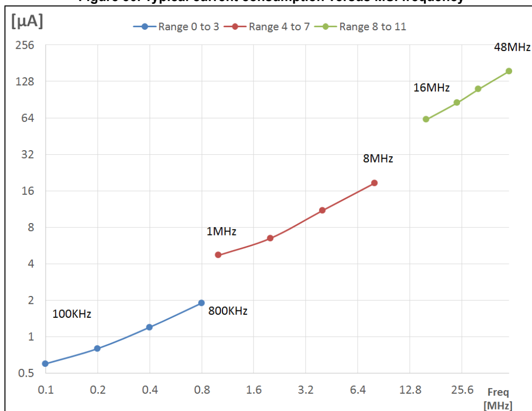
Figure 30. Typical current consumption versus MSI frequency
